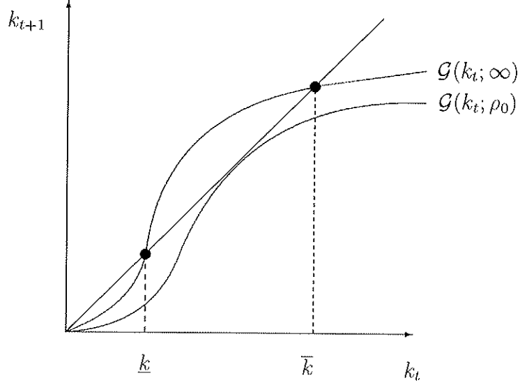
Figure 2: The saddle-node bifurcation
